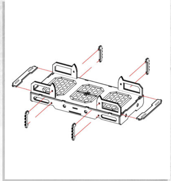
Walkway Assembly 2
