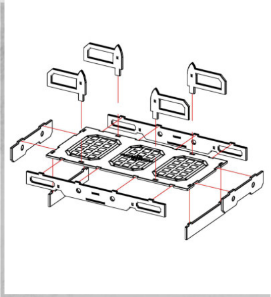
Walkway Assembly 1
