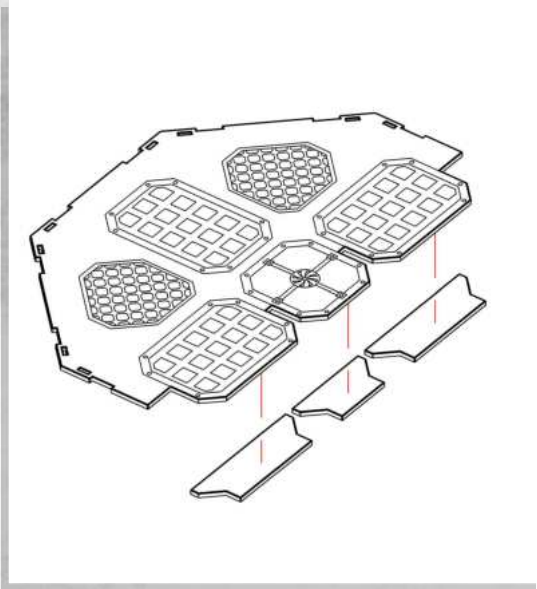
Platform Assembly 1
