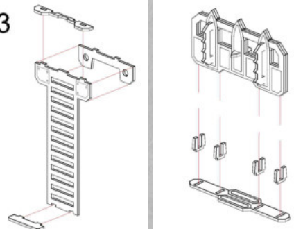
Accessory Assembly
