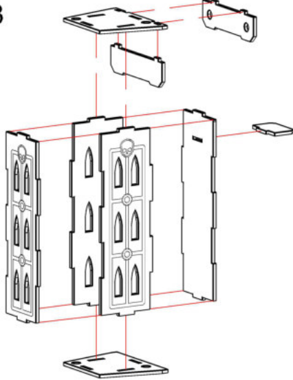
Tower Assembly
