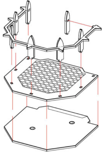
Tower Topper Assembly
