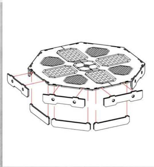
Platform Assembly 3
